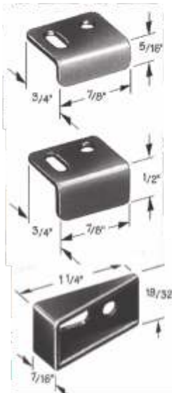
Strike Plate 5/16" Angle TMC100SP-19
